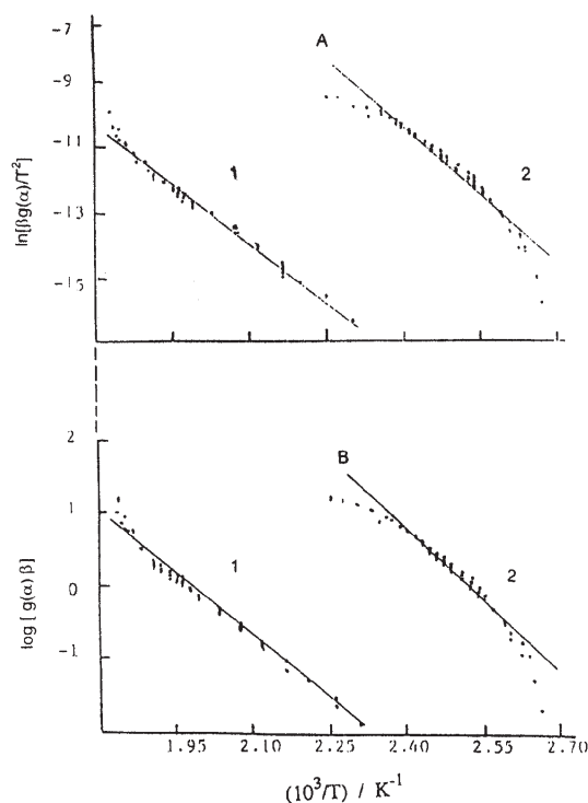
Fig. 5 Composite analysis of the dynamic TG data based on the modified Coats-Redfern equation (A) and Doyle's equation (B), assuming the contracting surface ( R_2 ) model. 1 – dehydration step; 2 – decomposition step
